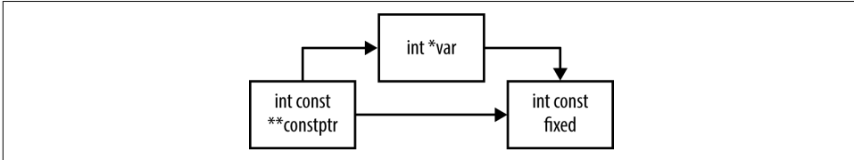
Figure 8-2. The links among the variables in Example 8-7
