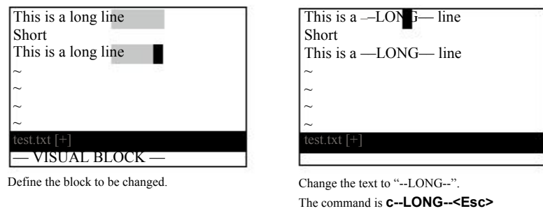
Figure 6.11 Block visual c command.
