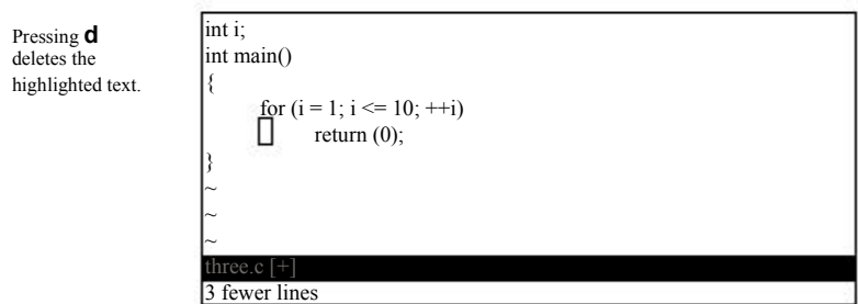
Figure 6.2 Visual delete.
