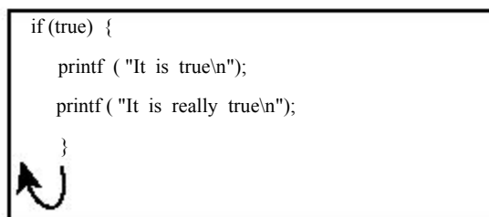
Figure 7.3 autoindent.
