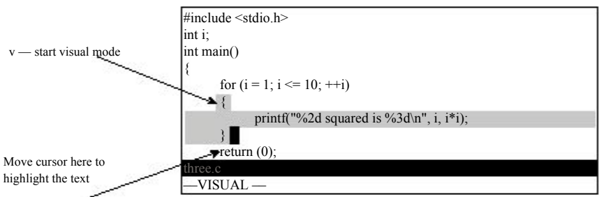
Figure 6.1 Visual mode.
