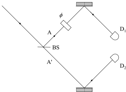
Fig. 1.4. An apparatus realizing a discrete two-beam experiment, in which detectors D_1 and D_2 are placed before the two orthogonal beams (A and A' ) can merge. “BS” indicates a 50–50 beam-splitter and “ \phi ” a variable phase-shifter.
