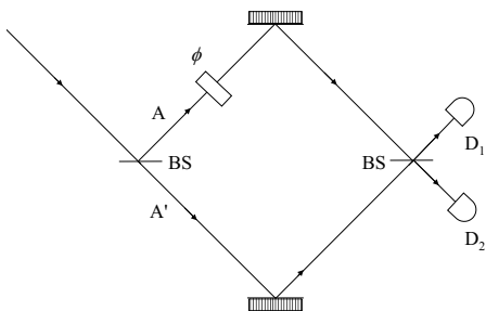
Fig. 1.5. Apparatus realizing a discrete two-beam experiment, in which detectors D_1 and D_2 are placed after the two orthogonal beams (A and A' ) have merged. This apparatus has the advantage over the original two-slit apparatus of Fig. 1.3 that no intensity is lost from the original beam during quantum state preparation. “BS” indicates a 50–50 beam-splitter and “ \phi ” a variable phase-shifter.
