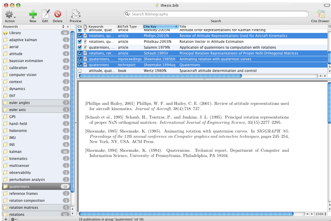
Figure 153 BibDesk
