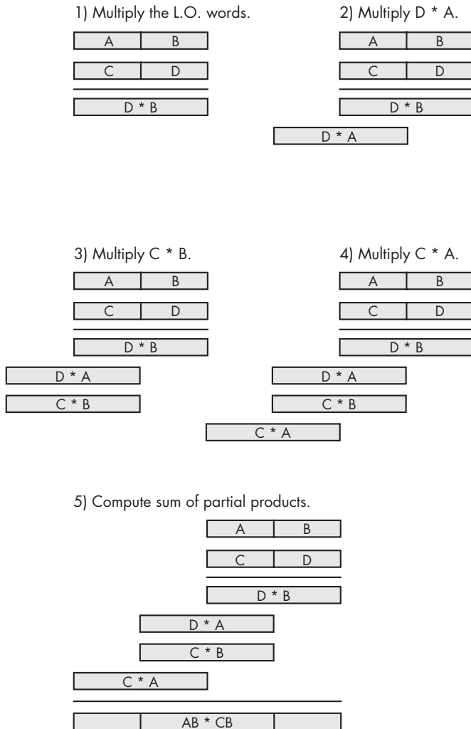
Figure 8-2: Extended-precision multiplication
