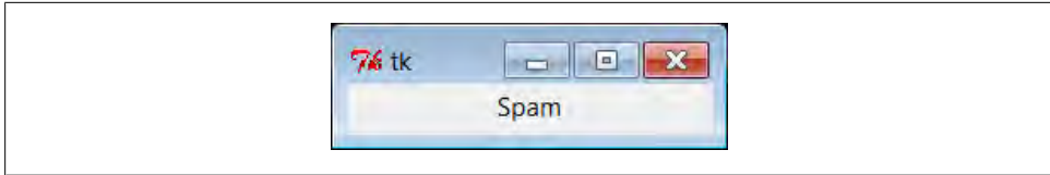
Figure 1-1. tkinter001.py window
