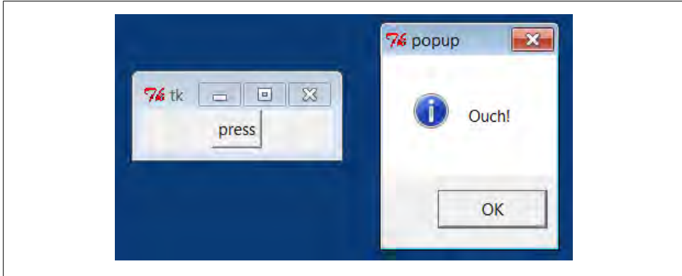
Figure 1-5. Customizing GUIs
