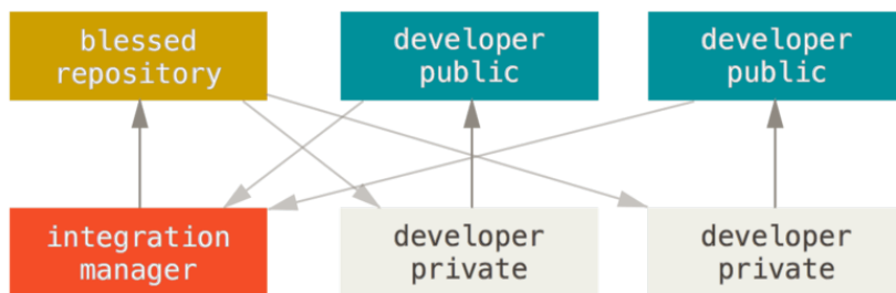
FIGURE 5-2 Integration-manager workflow.
