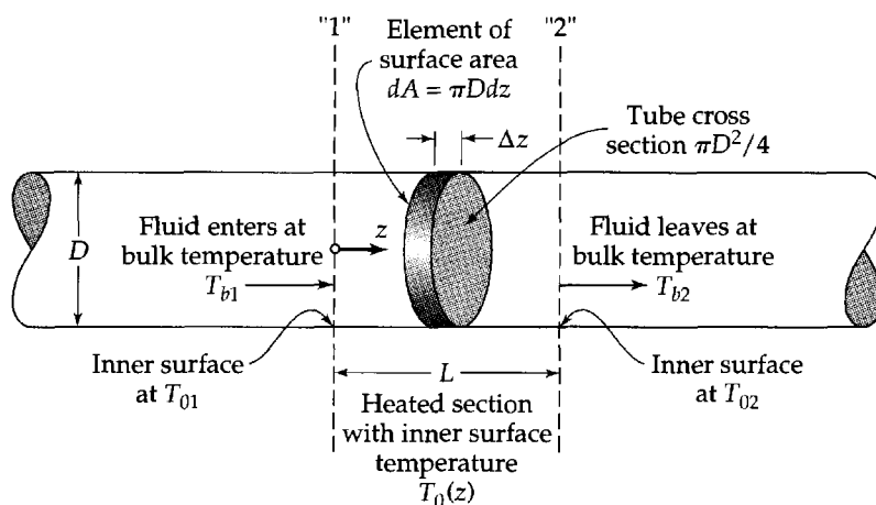
Fig. 14.1-1. Heat transfer in a circular tube.
