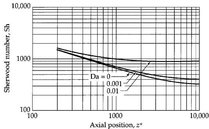
Fig. 21.4-1. Calculated Sherwood numbers, \text{Sh} = k_c D / \mathcal{D}_{AB} , for turbulent mass transfer from the wall of a tube, with and without homogeneous first-order chemical reaction. Results calculated at \text{Re} = 10,000 and \text{Sc} = 200 , as functions of axial position z^+ = zv_*/D and Damkohler number \text{Da} = k_1''' \nu / v_*^2 .
