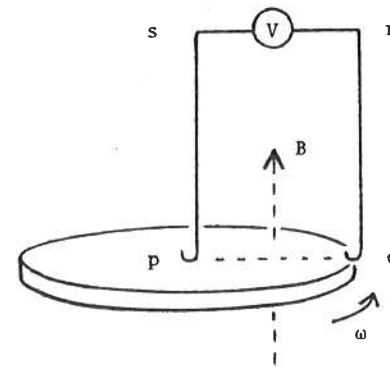
Fig. 7. Faraday's rotating disk experiment. The magnetic field B is perpendicular to the disk. The induced emf is registered on the volt meter.
