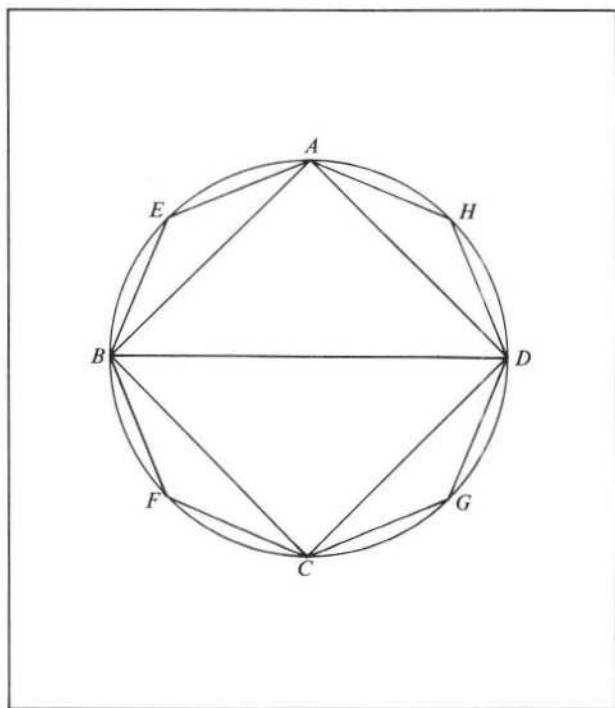
FIGURE 6. Book XII, Proposition 2, Exhaustion of a Circle
