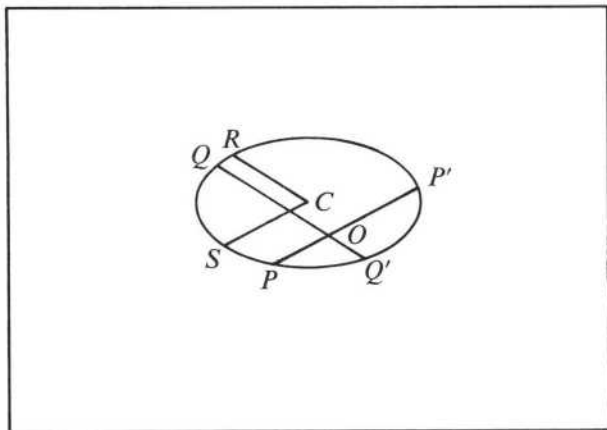
FIGURE 9. QO \cdot OQ' : PO \cdot OP' = CR^2 : CS^2
