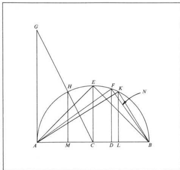
FIGURE 7. Book XIII, Proposition 18, Inscription of Regular Solids in a Sphere
