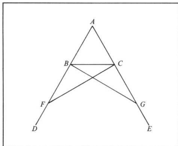
FIGURE 2. Book I, Proposition 5, Pons Asinorum
