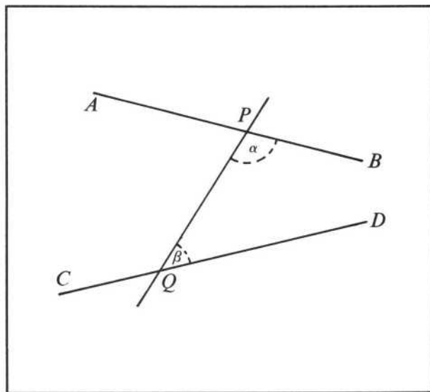
FIGURE 1. Book I, Postulate 5, \alpha + \beta < 2 Right Angles
