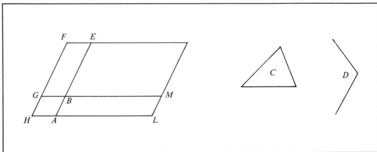
FIGURE 3. Book I, Proposition 44, Application of Areas
