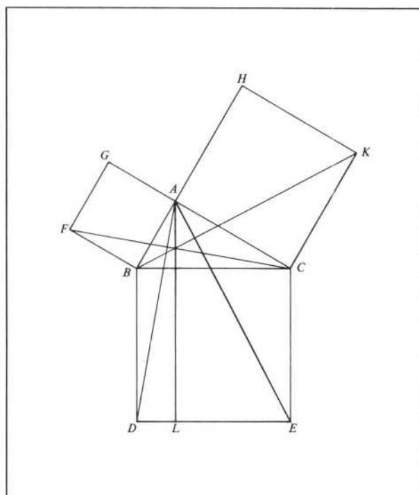
FIGURE 4. Book I, Proposition 47, "Pythagoras' Theorem," BC^2 = CA^2 + AB^2
