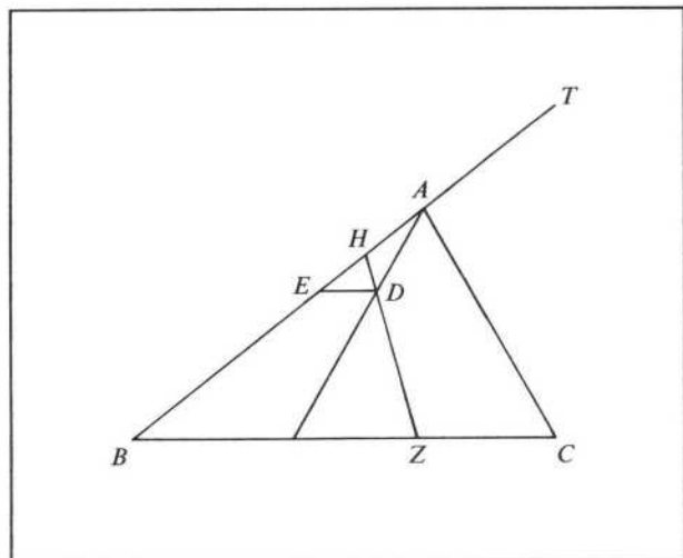
FIGURE 8. On the Division of Figures , Proposition 19
