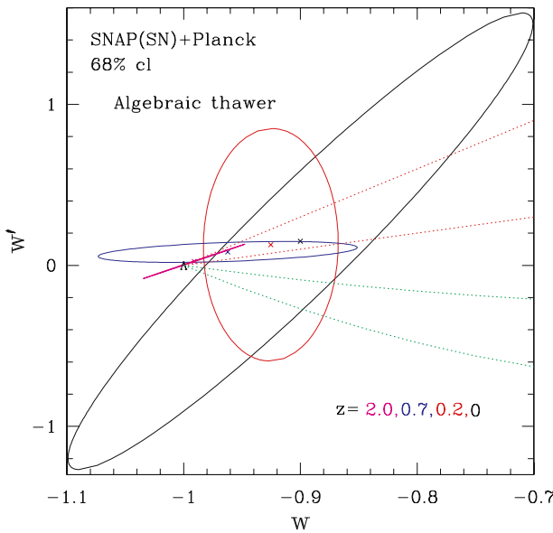
Fig. 6 As Fig. 4, for the algebraic thawing model
