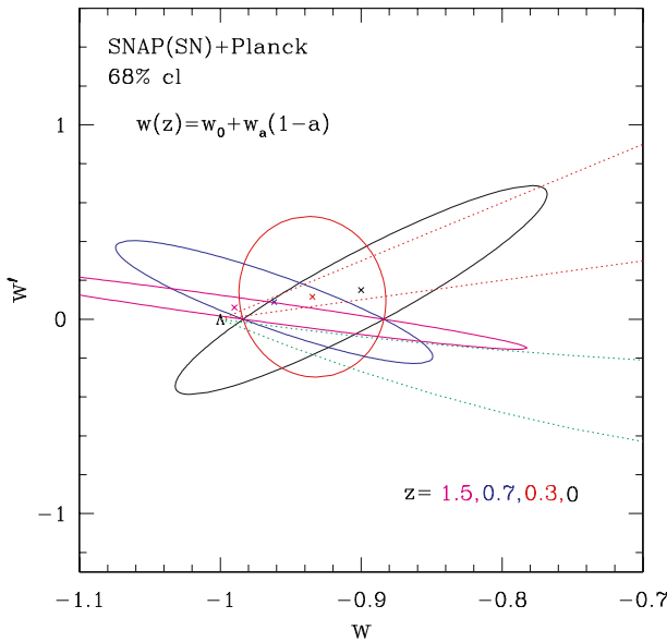
Fig. 4 Together with Figs. 5 and 6, this figure for the w_a thawing model illustrates constraints on the dynamical behavior of three thawing models at four redshift snapshots. While the z = 0 behavior is poorly limited by future data, taking into account the dynamical history still allows distinction of the fiducial w_0 = -0.9, w'_0 = 0.15 model from a cosmological constant and from the freezing class of physics
