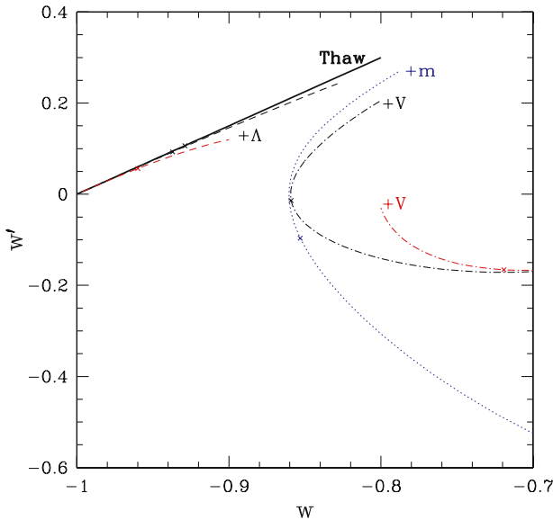
Fig. 2 Dynamics involving combination of physics can violate the fundamental phase space regions. To the original thawing scalar field trajectory ( solid black ), we add a cosmological constant ( +\Lambda ), extraneous matter or quartessence component ( +m ), or freezing scalar field ( +V ). We fix w_0 = -0.8 for the fields and take the total dimensionless dark energy density to be 0.7. For the second component of \Lambda or V we take \Omega_2 = 0.1 ( darker, black ) or 0.35 ( lighter, red ); for included matter \Omega_{+m} = 0.01 . Curve endpoints correspond to z = 0 , with x 's at z = 1
