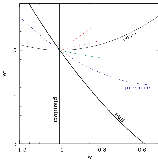
Fig. 1 The dynamical phase space w - w' is divided by three curves defined by physical conditions: the phantom line w = -1 , the null line w' = -3(1 - w^2) following from a flat potential, and the coasting line w' = 3(1 + w)^2 following from constant field velocity. These extend across the phase space. In addition, canonical dynamics leads to the distinct regions of the thawing regime bounded by the red dotted lines and the freezing regime bounded between the green dot-dashed curve and the blue dashed curve (the latter given by the constant pressure condition)
