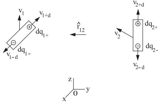
Figure 15.7: Two neutral current elements moving relative to the ground with velocities \vec{V}_1 and \vec{V}_2 .
