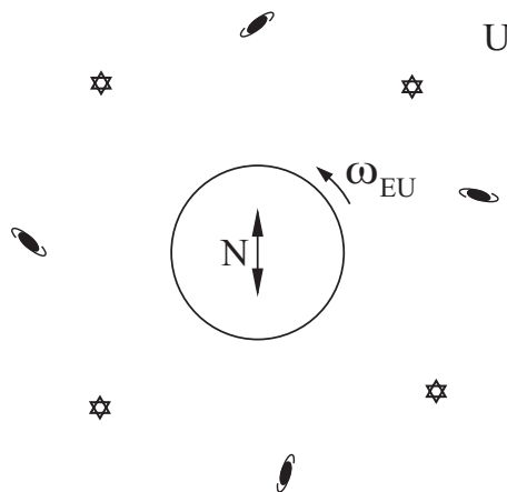
Figure 22.9: Plane of oscillation of Foucault's pendulum remains fixed relative to the frame of distant galaxies.
