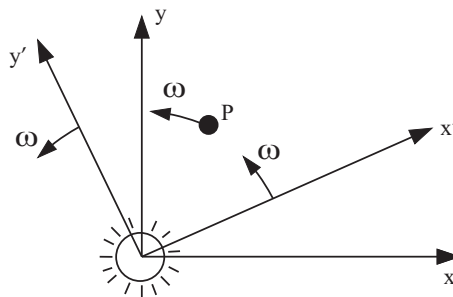
Figure 11.11: The non-inertial frame S' rotates relative to S together with the planet around the Sun.
