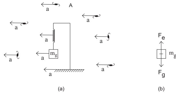
Figure 20.5: (a) Test body at rest in the ground suspended by a spring, as seen in frame A in with the test body, the spring, the Earth and the set of galaxies have the same common constant acceleration \vec{a} . (b) The gravitational force \vec{F}_g is balanced by the elastic force \vec{F}_e .
