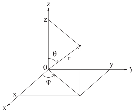
Figure B.3: Spherical coordinates (r, \theta, \varphi) .
