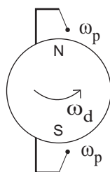
Figure 10.14: Earth spinning around its axis relative to absolute space or relative to an inertial frame of reference.
