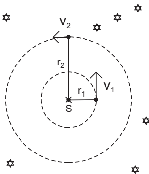
Figure 9.4: Two planets orbiting around the Sun.
