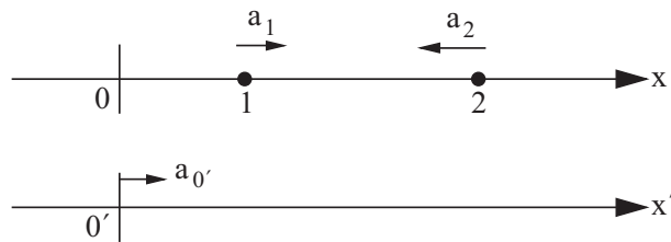
Figure 14.1: Accelerations a_1 and a_2 of two bodies relative to a frame of reference O . The frame O' has an acceleration a_{o'} relative to frame O .
