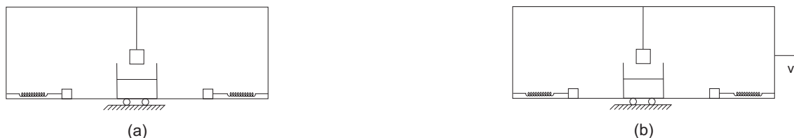
Figure 6.8: (a) Wagon at rest relative to the ground. (b) Wagon moving with a constant linear velocity v relative to the ground.
