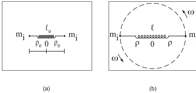
Figure 9.7: (a) Two globes at rest on the table separated by a distance l_0 . (b) Two bodies rotating with a common constant angular velocity \omega relative to the ground and separated by a distance l > l_0 .
