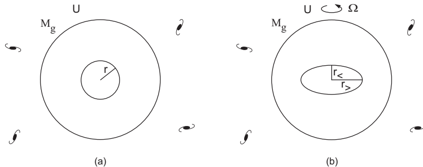
Figure 24.13: (a) Liquid drop of radius r surrounded by a rigid spherical shell of radius R > r . Both of them are at rest in the universal frame U . (b) New shape of the drop according to relational mechanics when only the rigid spherical shell rotates relative to U with a constant angular velocity around an axis passing through the center of the drop.
