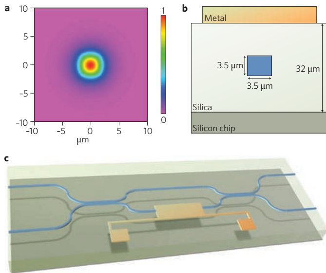
Figure 5 | Silica-on-silicon photonic quantum circuits. a , Light is guided in a waveguide much like in an optical fibre, as shown in this simulation of the transverse intensity profile. b , Schematic of a silica-on-silicon waveguide structure, showing the core (blue) and silica cladding. The metal heating element is lithographically patterned above the waveguide. c , A waveguide Mach-Zehnder interferometer, in which waveguide directional couplers can replace the bulk optics (beamsplitters) of Fig. 2. A metal element functions as a resistive heater that locally changes the refractive index — and thereby the phase — in one waveguide of the interferometer. Figures reproduced with permission from ref. 88, © 2009 NPG.
