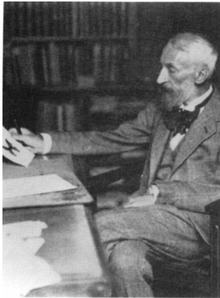
Figure 6: Eduard Study (1862 – 1930)
