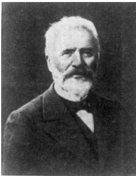
Figure 2: Camille Jordan (1838 – 1922)
